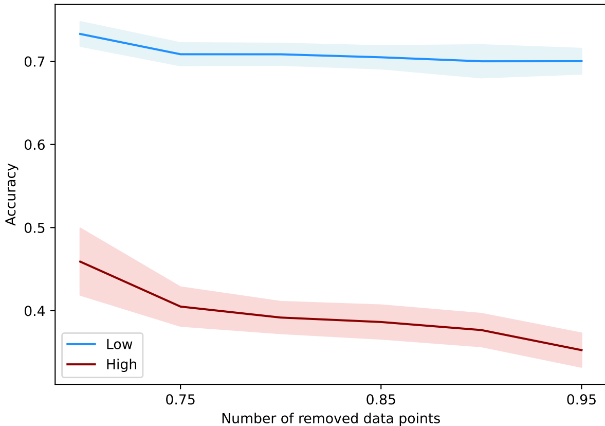
DataAttrOpt(3000, 0.03, 15, best, +b, alpha=best) - adult
